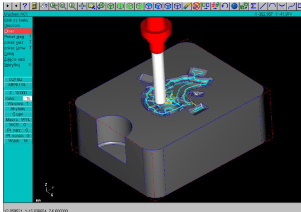
Fig. 3. Rough milling simulation in Mastercam.
