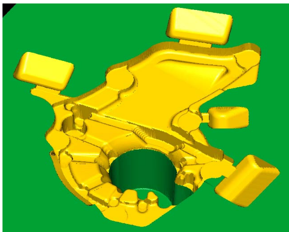
Fig. 4. Virtual model of movable die insert.
