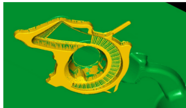
Fig. 5. Virtual model of fixed die insert.
